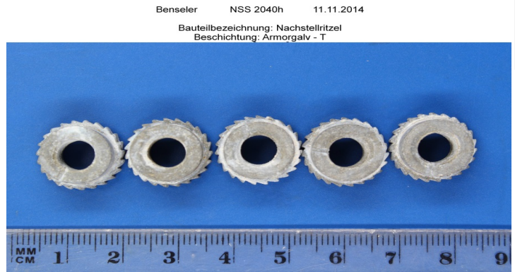
Sintered steel ratchet wheels (2040 Hrs salt spray)
