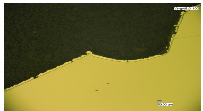
Cross section through the end of the thread
