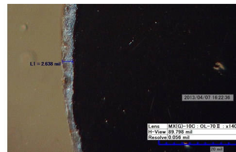
Figure 6 ArmorGalv ® after 3000 hours in salt fog environment
