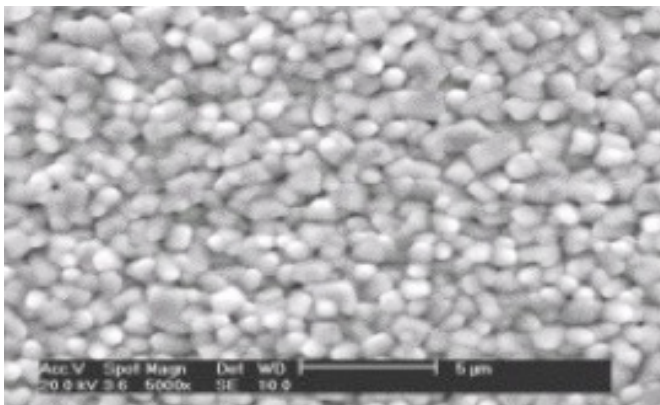
HDG surface showing a “sealed” structure
