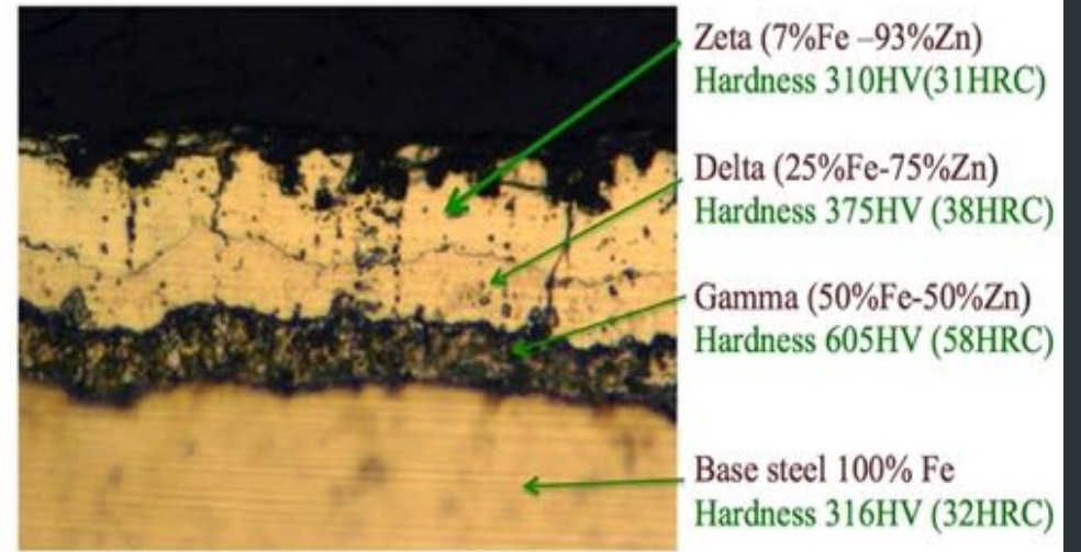
ArmorGalv® cross section
